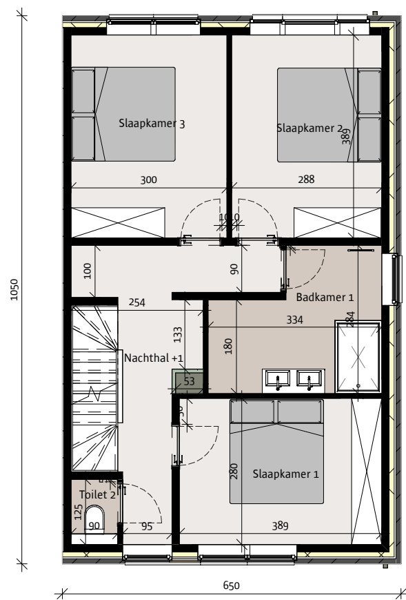
verdieping Opp. 68.25 m 2
