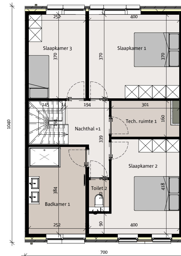
verdieping Opp. 72.8 m 2
